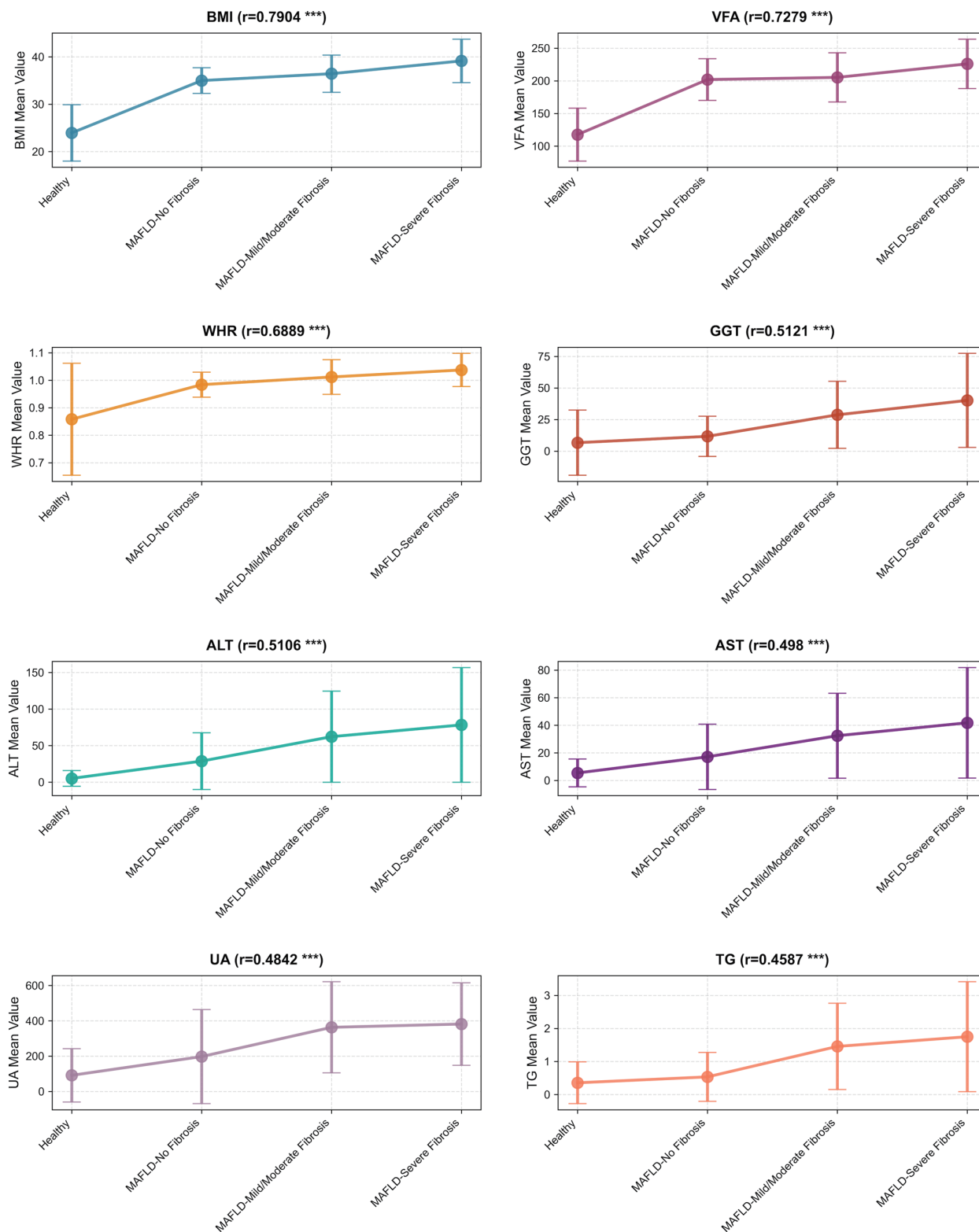
Fig. 6. Trends of metabolic indicators in healthy controls and MAFLD patients with different fibrosis progression. The top eight metabolic indicators with the strongest correlation are shown above, including anthropometric measurements (BMI, VFA, WHR), liver enzymes (GGT, ALT, AST), uric acid, and TG, all demonstrating a gradual increasing trend across advancing fibrosis stages in MAFLD. In the figure, r denotes the correlation coefficient; *** P < 0.001. MAFLD, Metabolic dysfunction-associated fatty liver disease; BMI, Body Mass Index; VFA, Visceral Fat Area; WHR, Waist-to-Hip Ratio; GGT, Gamma-Glutamyl Transferase; ALT, Alanine Aminotransferase; AST, Aspartate Aminotransferase; TG, Triglycerides.
